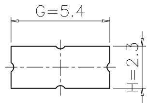
DETAIL "C" (S=5:1)
