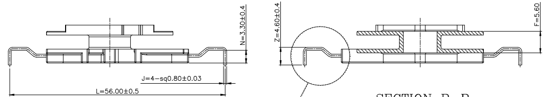
SECTION B-B
